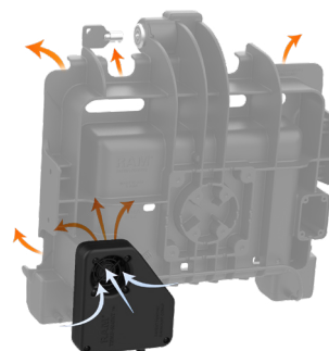
RAM-DOCK-HEATER1-AU P117-1022 RAM® Temp-Right™ Dock Heating Module for Zebra ET8x Tablet Docks
